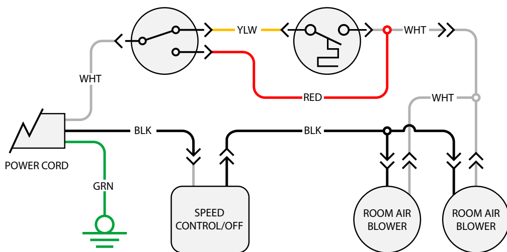
Figure 31B - ML300 Blower Wiring Schematic
