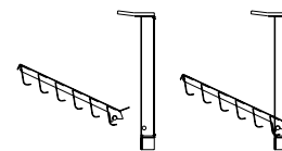
Bottom Louver Mounting Sequence
