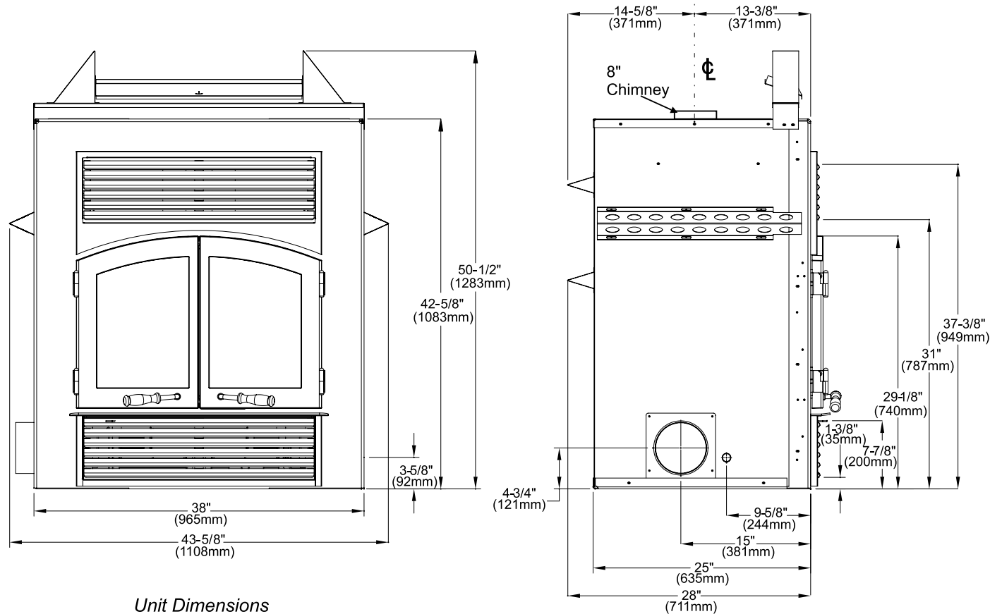
Unit Dimensions
