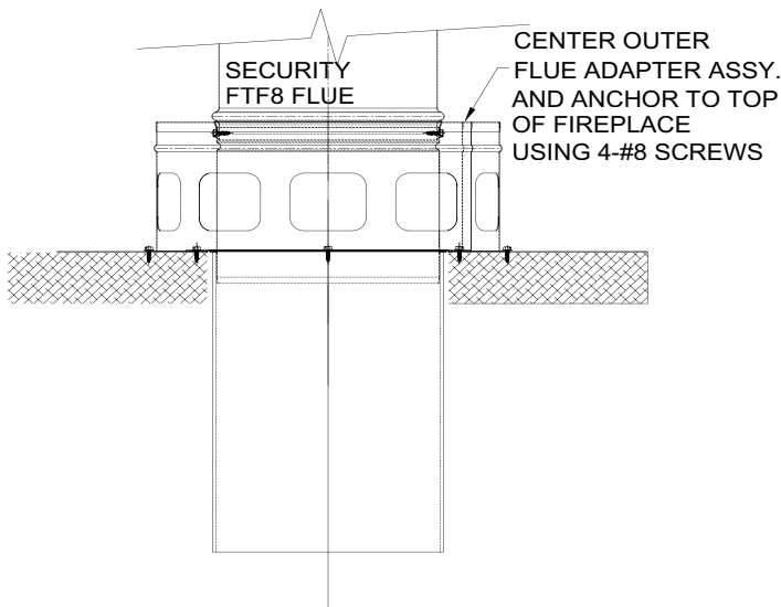
Security FTF8 Chimney System
