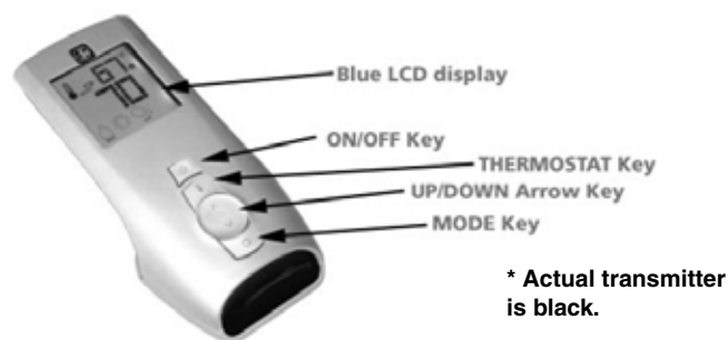
Figure 1: Proflame Transmitter
