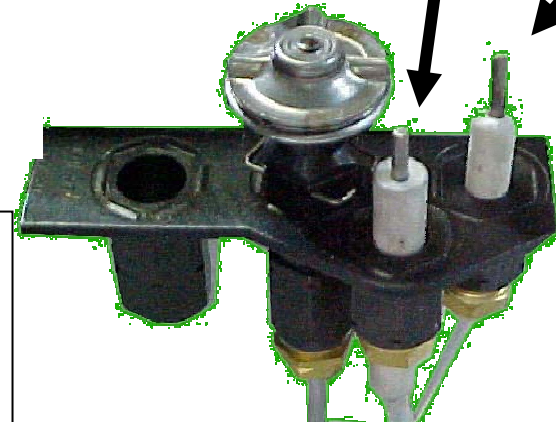
3 Way Pilot Assembly
