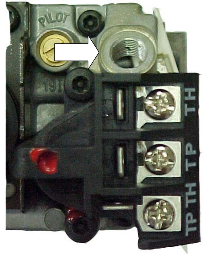
Standard SIT Valve
